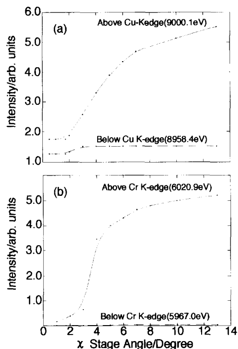
Fig. 2. The dependence of X-ray intensity emitted from the sample on angle \chi . The excitation energies were below and above the Cu K-edge for CuCl 2 (a) and below and above the Cr K-edge for Cr/SiO 2 catalyst (b).
